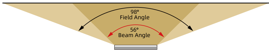
HORIZONTAL ANGLE
