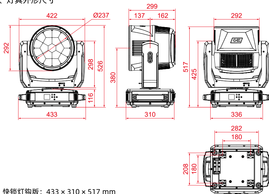
快锁灯钩版: 433 × 310 × 517 mm
